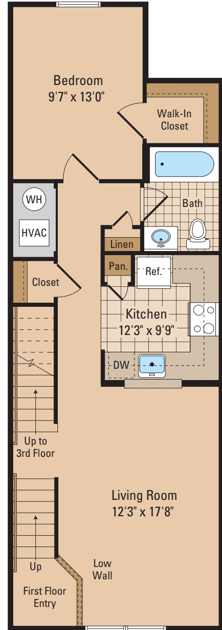
Second Floor
